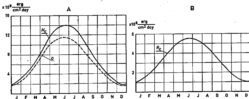
FIG. 3 VALUES OF H_c (FIGURE A) AND R_c (FIGURE B) DURING THE COURSE OF THE YEAR AT LATITUDE 52^\circ .
