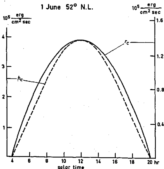
FIG. 2 VALUES OF h_c AND r_c ON A PERFECTLY CLEAR DAY ON 1st JUNE AT LATITUDE 52^\circ .
