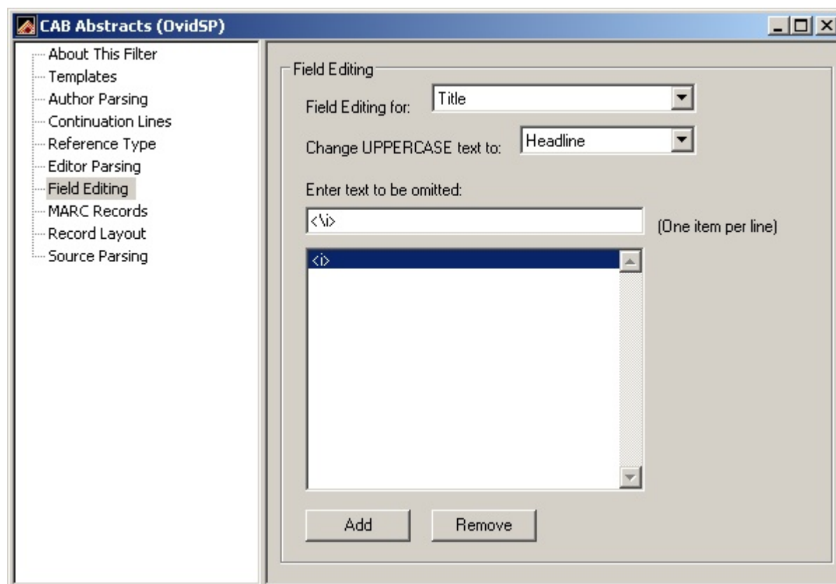
Figure 19. The Field editing window in the Filter editor
