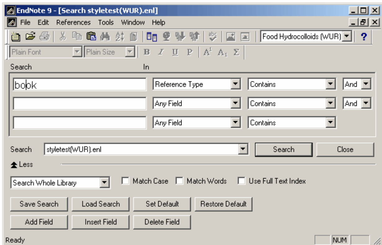
Figure 35. Search window
