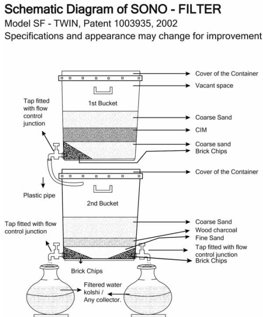
Fig. 2. Schematic diagram of Sono 2-bucket filter (Hussam et al. , 2008) (left); picture of Sono filter taken by one of the authors (right).
