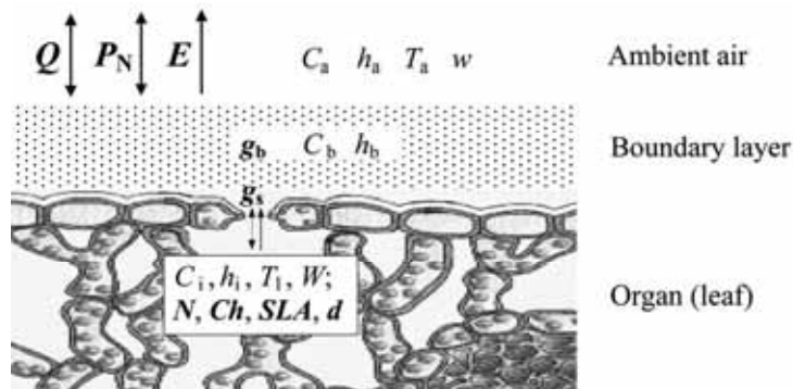
Figure 1. Photosynthetic apparatus of a leaf, gas and radiative-energy fluxes, input variables and state variables related to the GREM. Q is total radiation flux (photosynthetically active ( Q_p ), near infrared and thermal infrared), P_N and E are net photosynthesis and transpiration rate, respectively, C_a , C_b , C_i and h_a , h_b , h_i are \text{CO}_2 content and relative humidity of ambient air (subscript a), of air within leaf boundary layer (subscript b), or of the air within leaf intercellular spaces (subscript i), respectively. T_a and T_i are the temperature of the ambient air and of the leaf, g_s and g_b are stomatal and boundary-layer conductance, and w is the wind speed of ambient air. W is leaf water potential, and N and Ch are leaf nitrogen and chlorophyll concentration per unit leaf area, respectively. SLA is specific leaf area (area per unit mass) and d is leaf width. The ellipsoid structures are the chloroplasts representing distributed sites of photochemical conversion of light energy and biochemical \text{CO}_2 fixation within mesophyll cells. The transport of \text{CO}_2 between intercellular spaces and reaction sites in the liquid phase of mesophyll cells is not considered in the scheme
