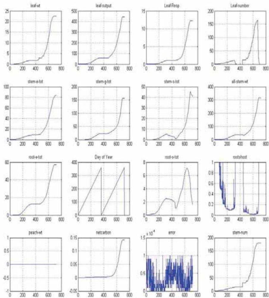
Figure 2. Sample output of quantitative data generated by L-PEACH and visualized using MATLAB after a simulation run. As indicated on the X axis these data are for a simulation of two years. The graphs make it possible for the user to track and quantitatively analyse various aspects of the model behaviour over time
