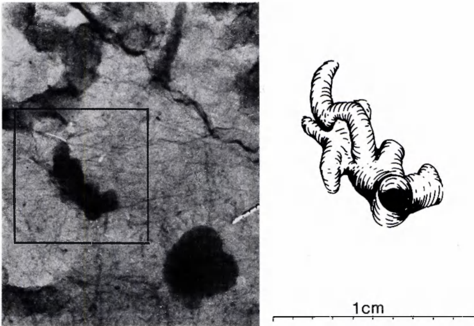
Fig. 6. Multiple branching worm channel made by an Allolobophora species; from about 4 cm depth in grass strip at control plot. Excision and drafted interpretation from a radiograph of 5 mm thick, vertically oriented soil section.
