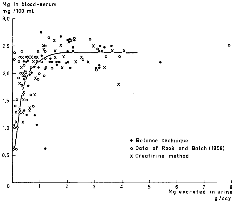
FIG. 1. Correlation between the daily amount of magnesium excreted in urine and the magnesium concentration in blood-serum
