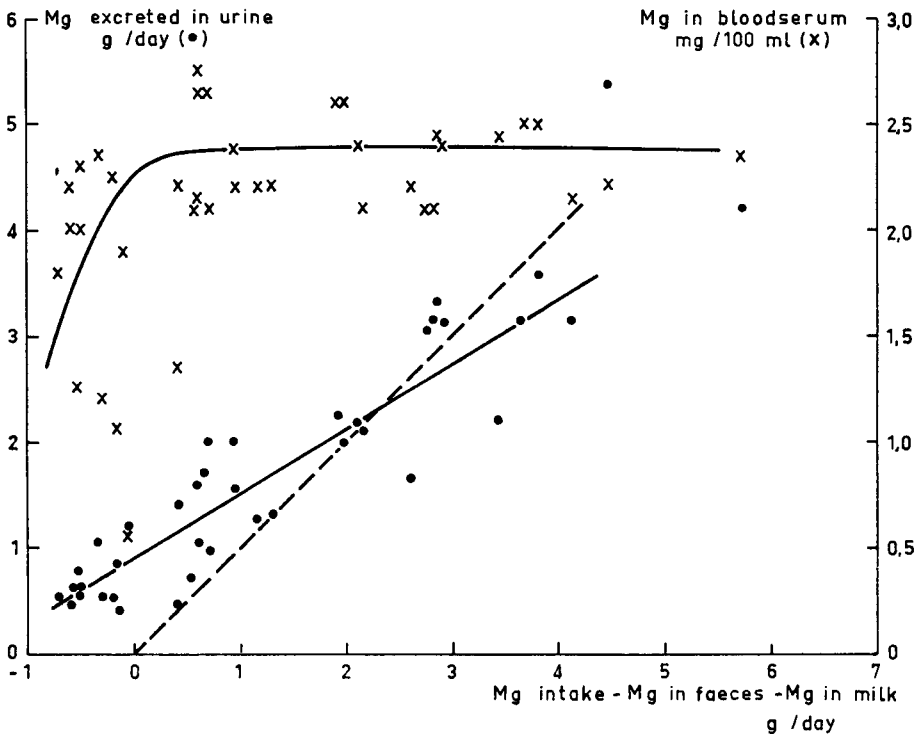
FIG. 2. Correlation between the amount of "available" magnesium above the quantity secreted in milk (g/day) and the amount of magnesium excreted in urine (g/day) and the serum magnesium concentrations (mg/100 ml)
