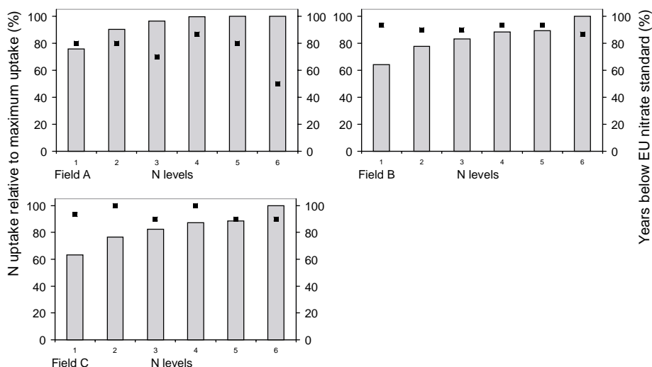
Figure 3. Average relative N uptake (bars – left y-axis) and percentage of years in which the EU standard of 50 \text{ mg l}^{-1} was not exceeded (square points – right y-axis). Data presented for 6 N application levels and three fields with a different land use history. Field A: old pasture; field B: reseeded pasture; field C: previously cropped to maize. Values for N uptake are relative to the N uptake at the highest N level for field A (100%).
