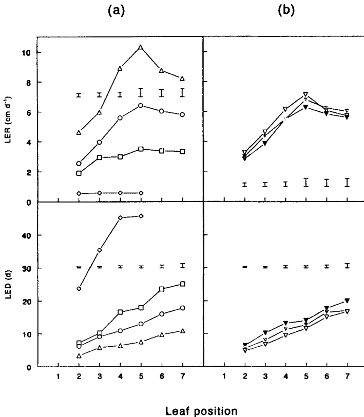
Figure 4. LER and LED of Leaves 2–7, (a) averaged per temperature treatment and (b) averaged per PPFD treatment. Symbols 13/8°C: ◇; 18/13°C: □; 23/18°C: ○; 28/23°C: △; dark (inversed) triangle: 104 \mu\text{mol m}^{-2} \text{s}^{-1} ; grey triangle 185 \mu\text{mol m}^{-2} \text{s}^{-1} ; open triangle: 277 \mu\text{mol m}^{-2} \text{s}^{-1} . Bars indicate the LSD ( P = 0.05 ).
