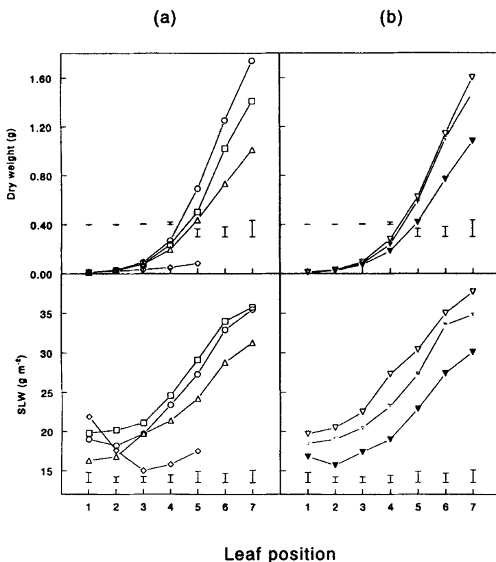
Figure 3. Dry weight and SLW of Leaves 1–7, (a) averaged per temperature treatment and (b) averaged per PPFD treatment. Symbols: 13/8^\circ\text{C} : ◇; 18/13^\circ\text{C} : □; 23/18^\circ\text{C} : ○; 28/23^\circ\text{C} : △; dark (inversed) triangle: 104 \mu\text{mol m}^{-2} \text{s}^{-1} ; grey triangle 185 \mu\text{mol m}^{-2} \text{s}^{-1} ; open triangle: 277 \mu\text{mol m}^{-2} \text{s}^{-1} . Bars indicate the LSD ( P = 0.05 ).
