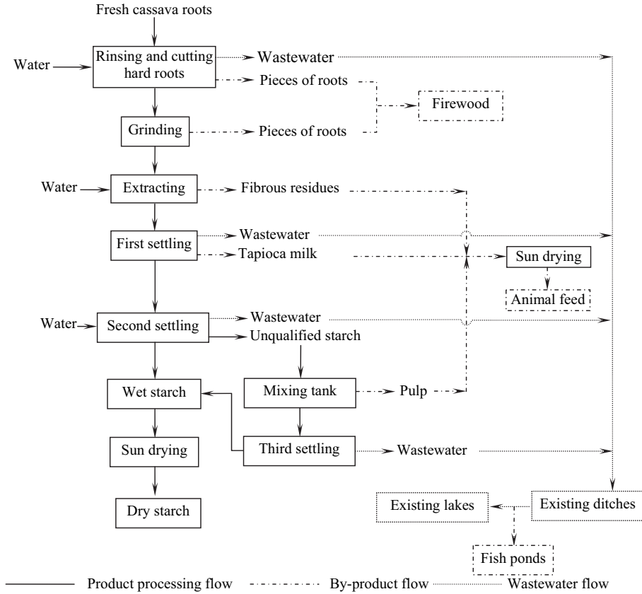
Figure 2. Diagrammatic representation of the family-scale tapioca production process at Tra Co Village, Vietnam.
