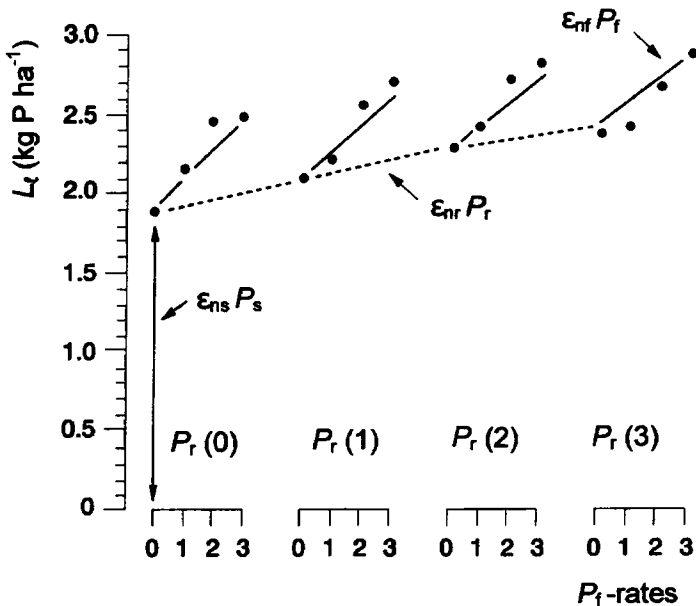
Figure 5. P uptake by lentil L_t (kg P ha -1 ) in response to residual ( P_r ) and directly applied P fertilizer ( P_f ), both at rates of 0 (0), 17.5 (1), 35.0 (2) and 52.5 (3) kg P ha -1 , at Breda for harvest 1987. Actual P-uptake is denoted by solid dots (Table 4). The intersect with the y-axis represents Equation 4 with \epsilon_{nls} = 0.0634 and P_s = 4.8 , at P_r = P_f = 0 . The broken line represents Equation 4 for \epsilon_{nr} = 0.00035 and P_r rates from (0) to (3), at P_f = 0 . The solid lines represent Equation 4 for \epsilon_{nr} = 0.00035 and P_f rates from (0) to (3).
