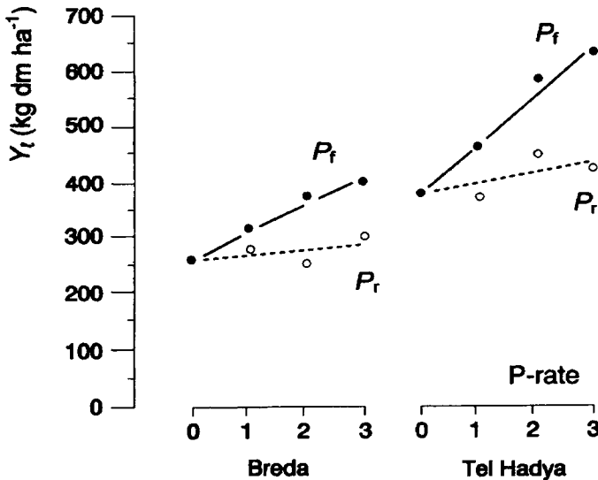
Figure 3. Yield response of lentil at early vegetative stage Y_{\ell} (kg DM ha -1 ) to directly applied ( P_f ) and residual P ( P_r ) from fertilizer at rates of 0 (0), 17.5 (1), 35.0 (2) and 52.5 (3) kg P ha -1 at Breda and Tel Hadya during the 1986/87 growing season (Table 4). Open circles refer to the P0res-P3res at P0dir treatments, and dots to P0dir-P3dir at P0res treatments (Table 4). Solid and broken lines represent simple linear regression equations.
